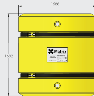
DBM - PE Skin, Ultralight Carbon Foam Dry Weight: 1,603 kg EOL Uplift: 1,296 kg
