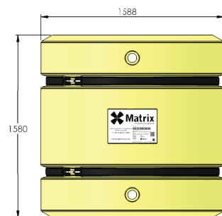
DBM - GRP Skin, Ultralight Carbon Foam Dry Weight: 1,415 kg EOL Uplift: 1,293 kg
